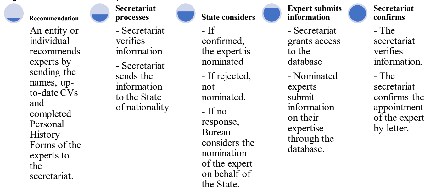
Figure 2: Recommendation process
