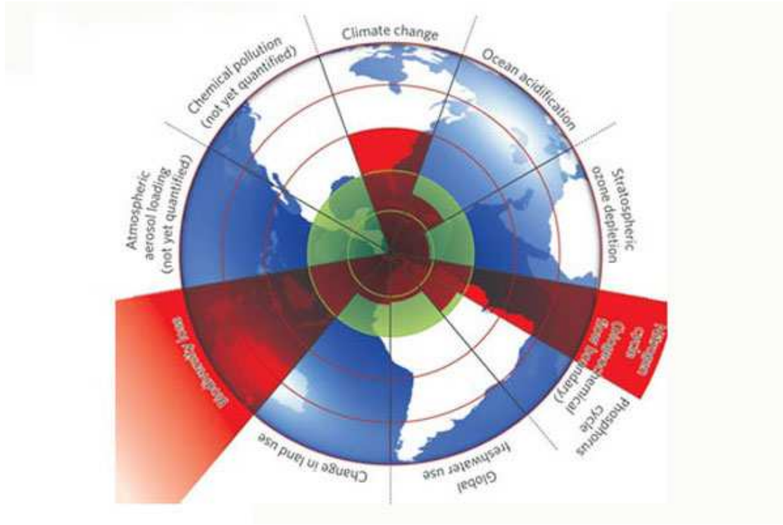
Figure 1. The nine planetary boundaries
