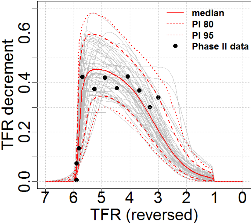
Double-logistic decline function
