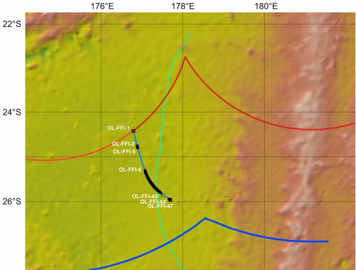
Figure 1: Map showing the outer limit line and provisions of article 76 invoked (light blue line) of Fiji in the Lau Ridge – northern South Fiji Basin Region. Further indicated are: The 200 M line of Fiji (red line), the 350 M line (dark blue line), and the 2500 m isobaths plus 100 M (green line)
